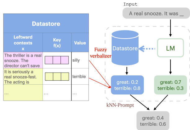
Figure 1: kNN-Prompt incorporates information from a large, heterogeneous corpus to facilitate zero-shot inference. The datasore contains key-value pairs where the key is an encoding of a leftward context and the value is the next token following the context.
